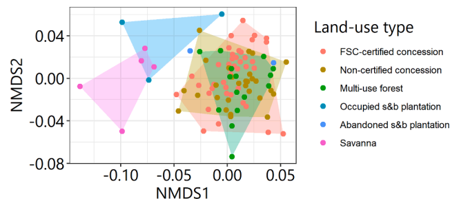
Fig. 4. NMDS ordination of the soundscapes recorded in various land-use types, using the soundscape dissimilarity index. Colored shapes indicate convex hulls. FSC certified logging concession (n = 41), non-certified logging concession (n = 28), multi-use forest (n = 15), occupied slash and burn plantation (n = 3), abandoned slash and burn plantation (n = 2) and savanna (n = 5).
